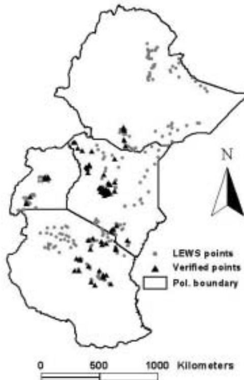
Figure 1: Location of the LEWS monitoring sites and verification sites in East Africa.
